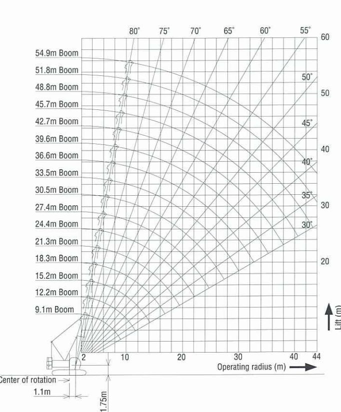
Boom Working Range
