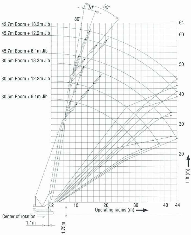
Fixed Jib Working Range
