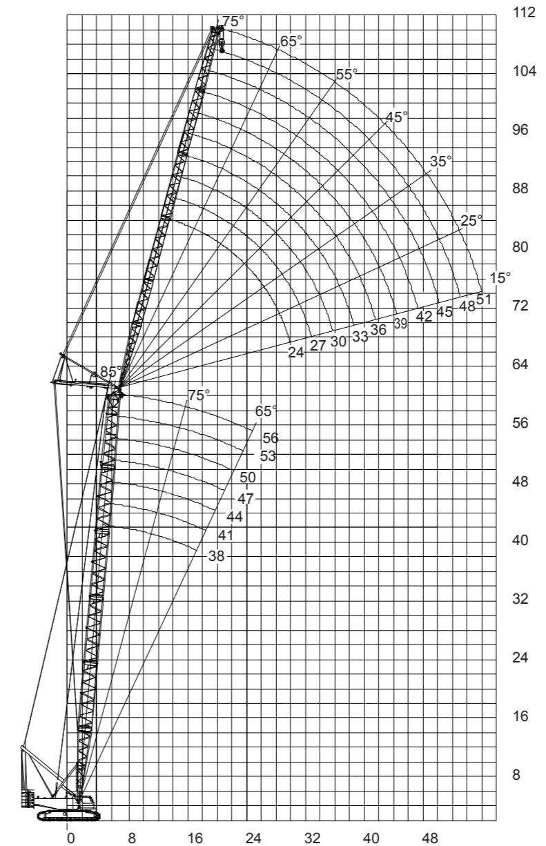
Luffing Fly Jib Lifting Height Curve
