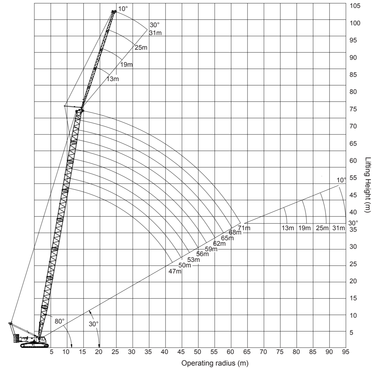
Fixed Fly Jib Lifting Height Characteristics Curve
