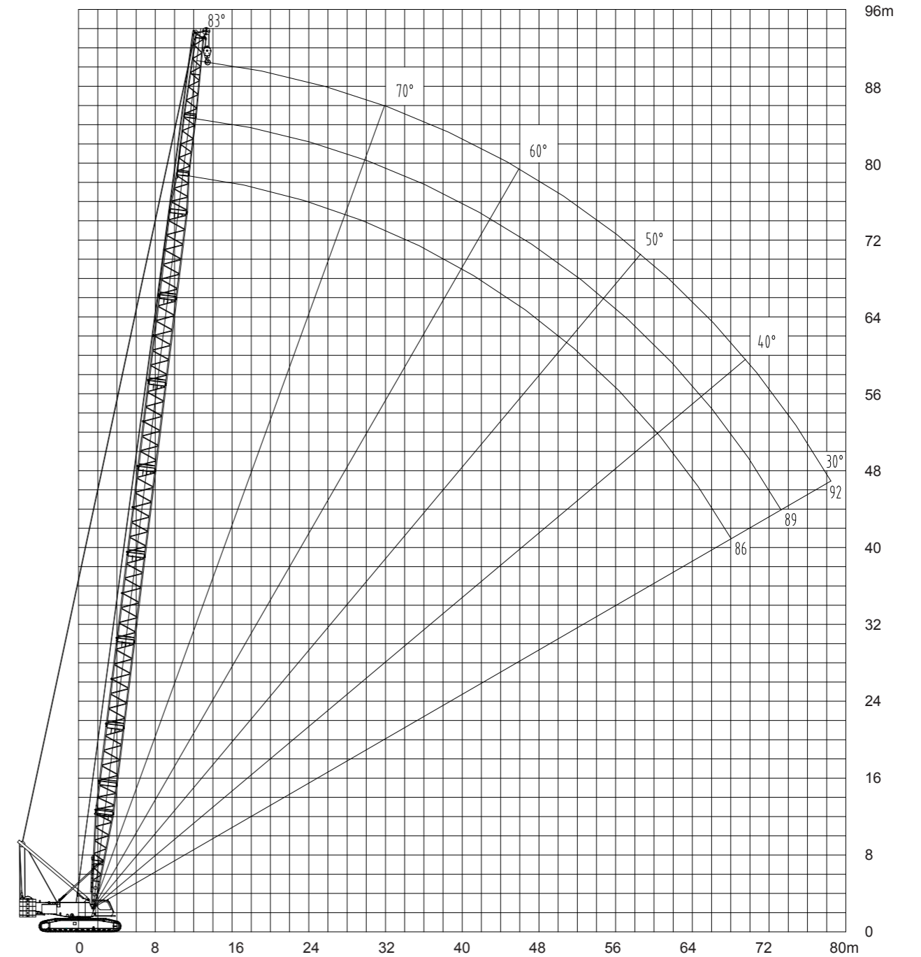
Light Duty Boom Lifting Height Characteristics Curve
